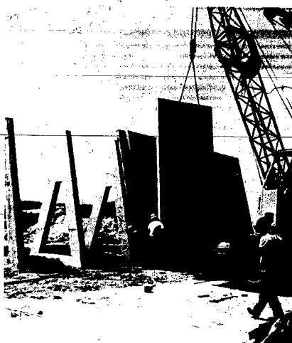
A PRE-CAST WALL PANEL for the "Husker" silo is being lifted into position by the crane at right. The wall panel is supported on pre-cast concrete buttresses (triangular structures at left).
